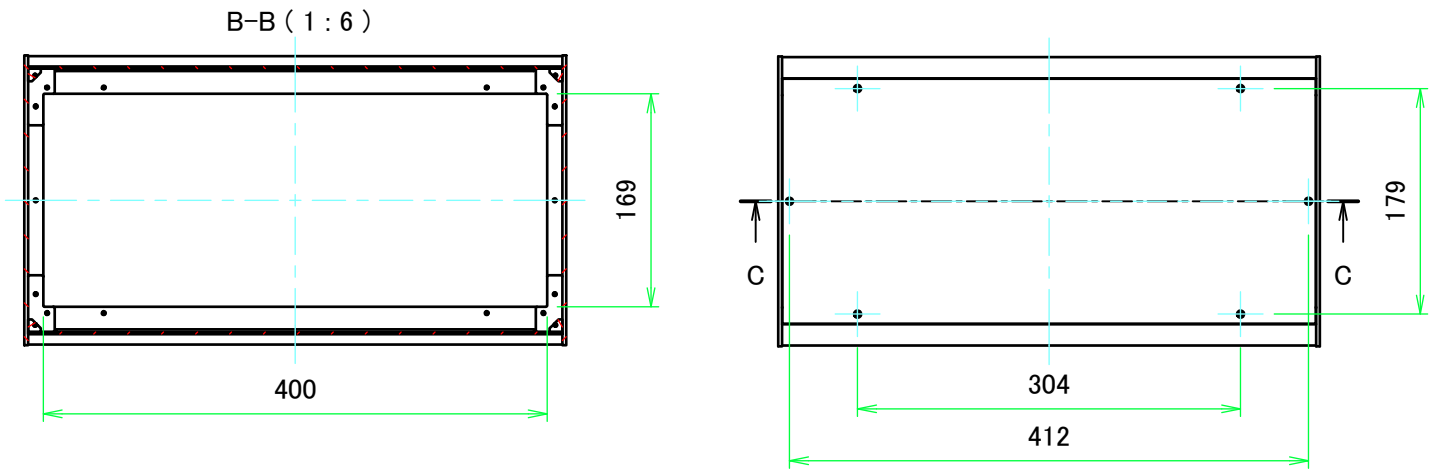
E view
